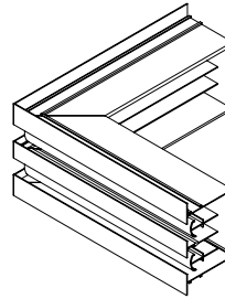
STACK MITER (OUTSIDE)
