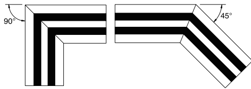
FACE MITER 90° AND 45°
